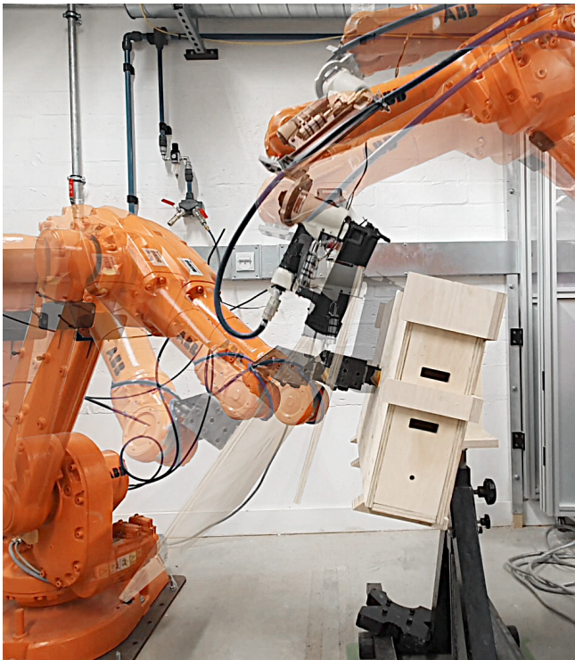
Figure 2. Robotic Assembly of Architectural Parts. Image: Kevin Saey.
